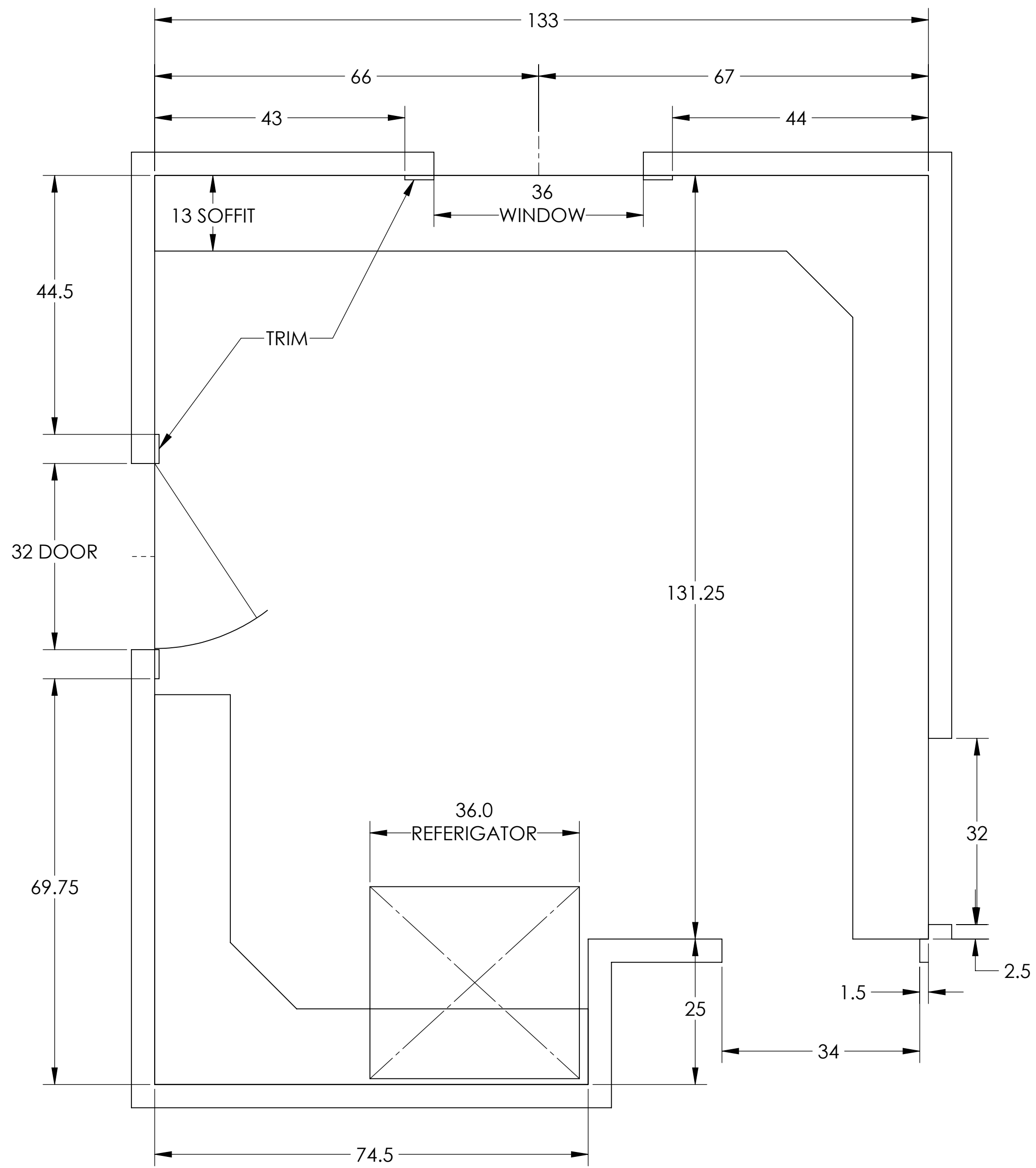
WALL LAYOUT
